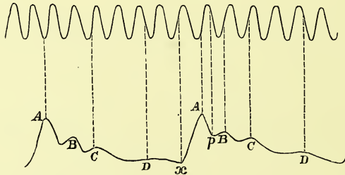
Fig. 49. PULSE-TRACING FROM CAROTID ARTERY OF HEALTHY MAN (from Moens).
